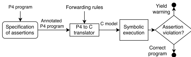
Figure 2: Overview of ASSERT-P4.
